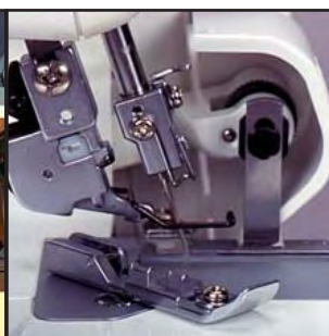
Multi-Purpose Foot comes equipped with a slotted tape guide which can be used to sew woven tape, elastic, sequins and ribbon.
