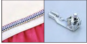
Elasticator Presser Foot: Part No. A9815-655-0A0A
